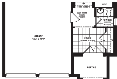
PARTIAL GROUND FLOOR ELEV. 'B'
