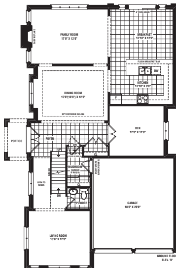
GROUND FLOOR ELEV. B
